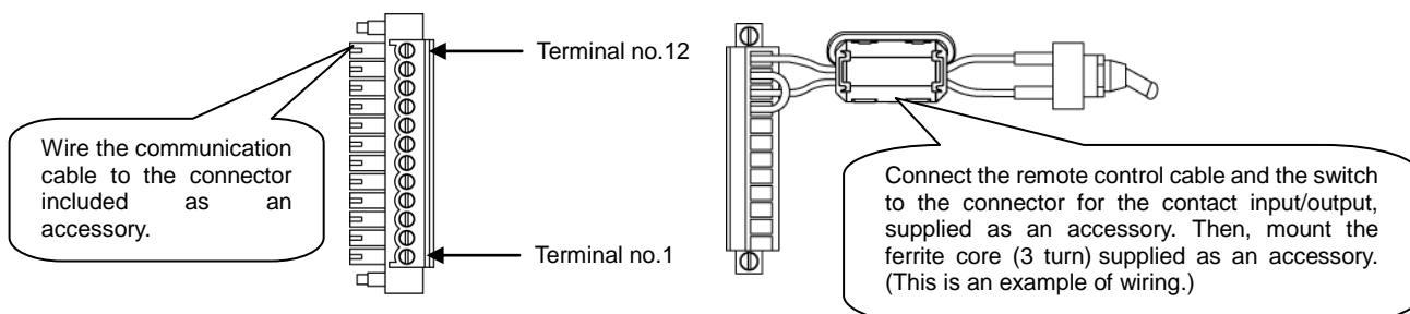
Fig 2.3-2 Attached connector and terminal no (Example)
